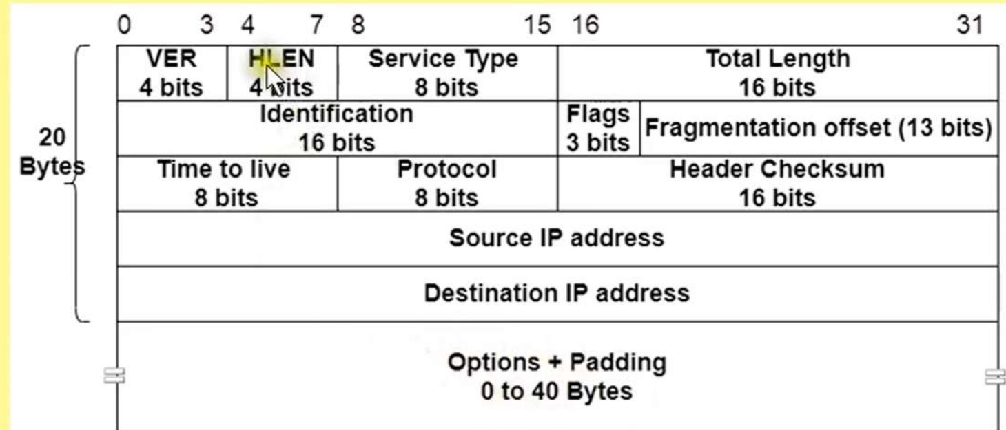
IP Header Format
