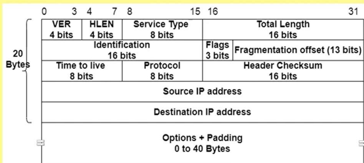
IP Header Format
