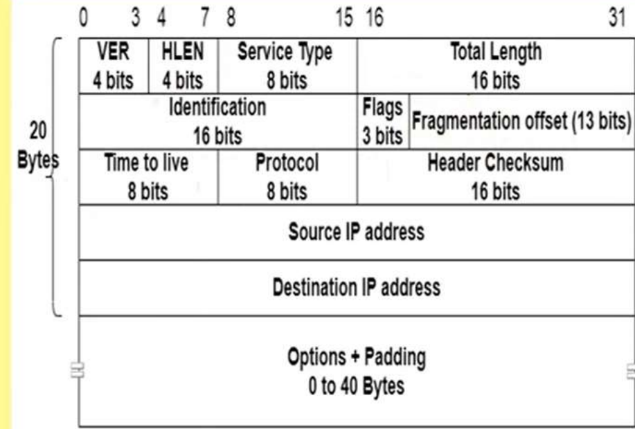
IP Header Format
